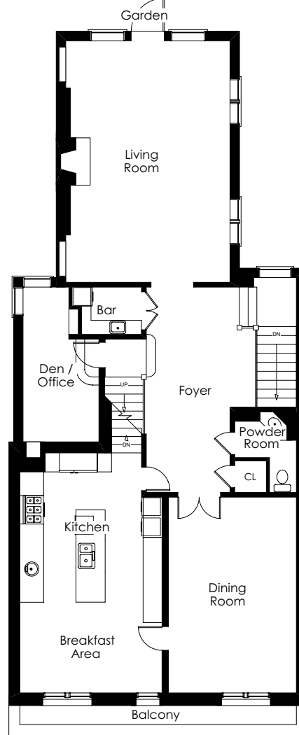
Main Floor
