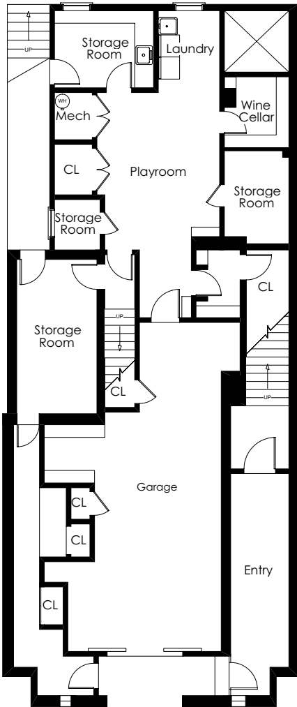
Lower Floor
