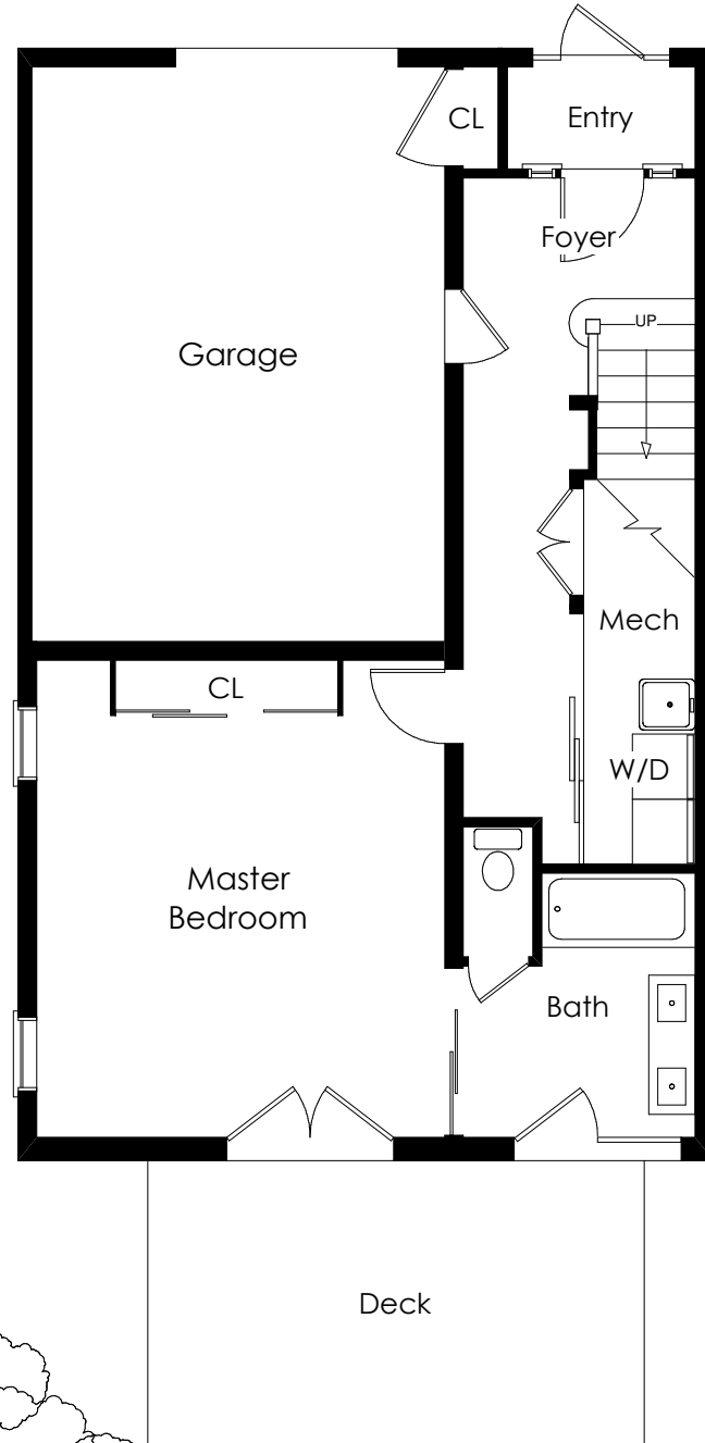
Lower Floor
